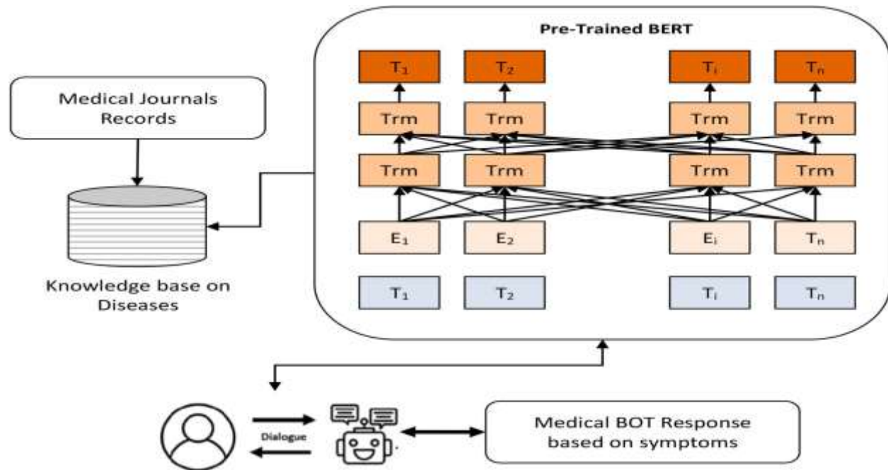
Figure 3: Proposed design for BERT base medical BOT
