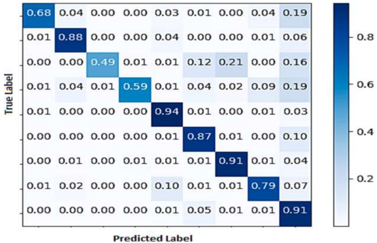
Figure 5: Confusion matrix of proposed model
