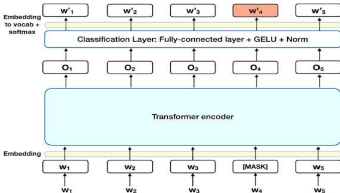
Figure 2: Generic BERT-architecture
